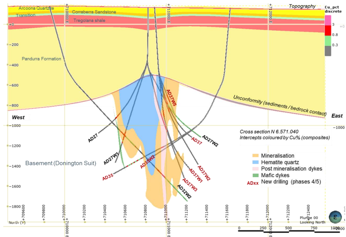
Figure 3. Representative cross-sections (A-A' from Figure 2.) showing simplified geology and down hole Cu assays.
